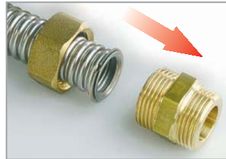
Remove union nipple to inspect flat-sealing surface.
