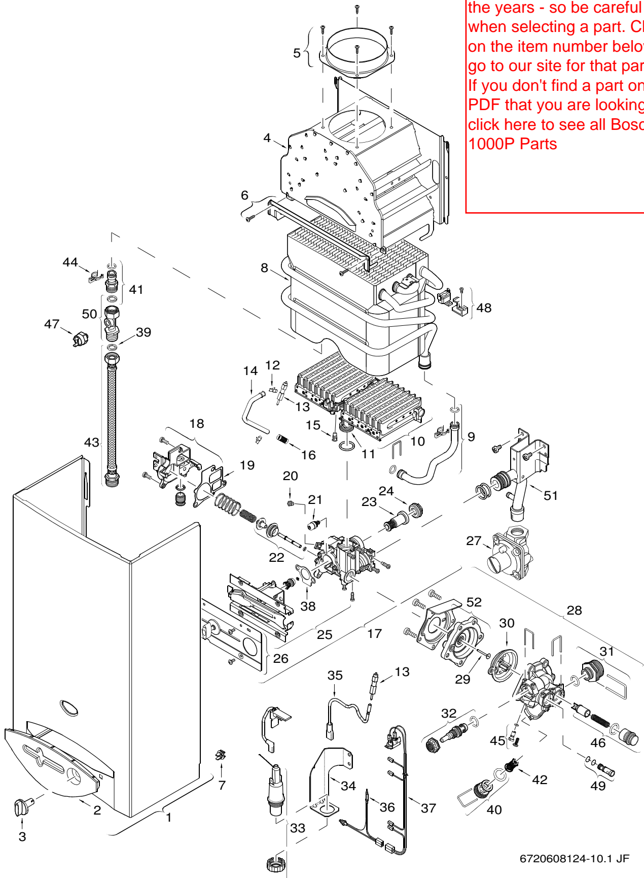
Fig. 28 Components Diagram
