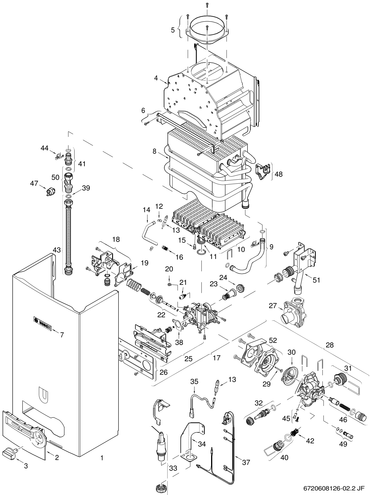
Fig. 29 Components Diagram
