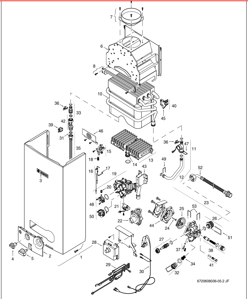
Fig. 27 Components Diagram
