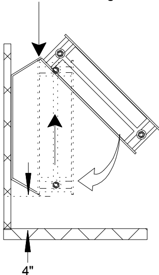
Step # 4 Radiator mounting on bracket.
