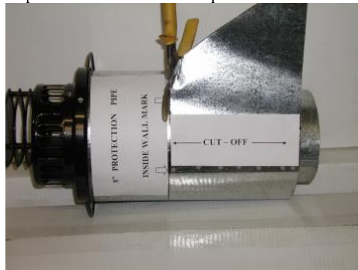
Step 4 – Cut off 8” Protection Pipe excess at wall mark.
